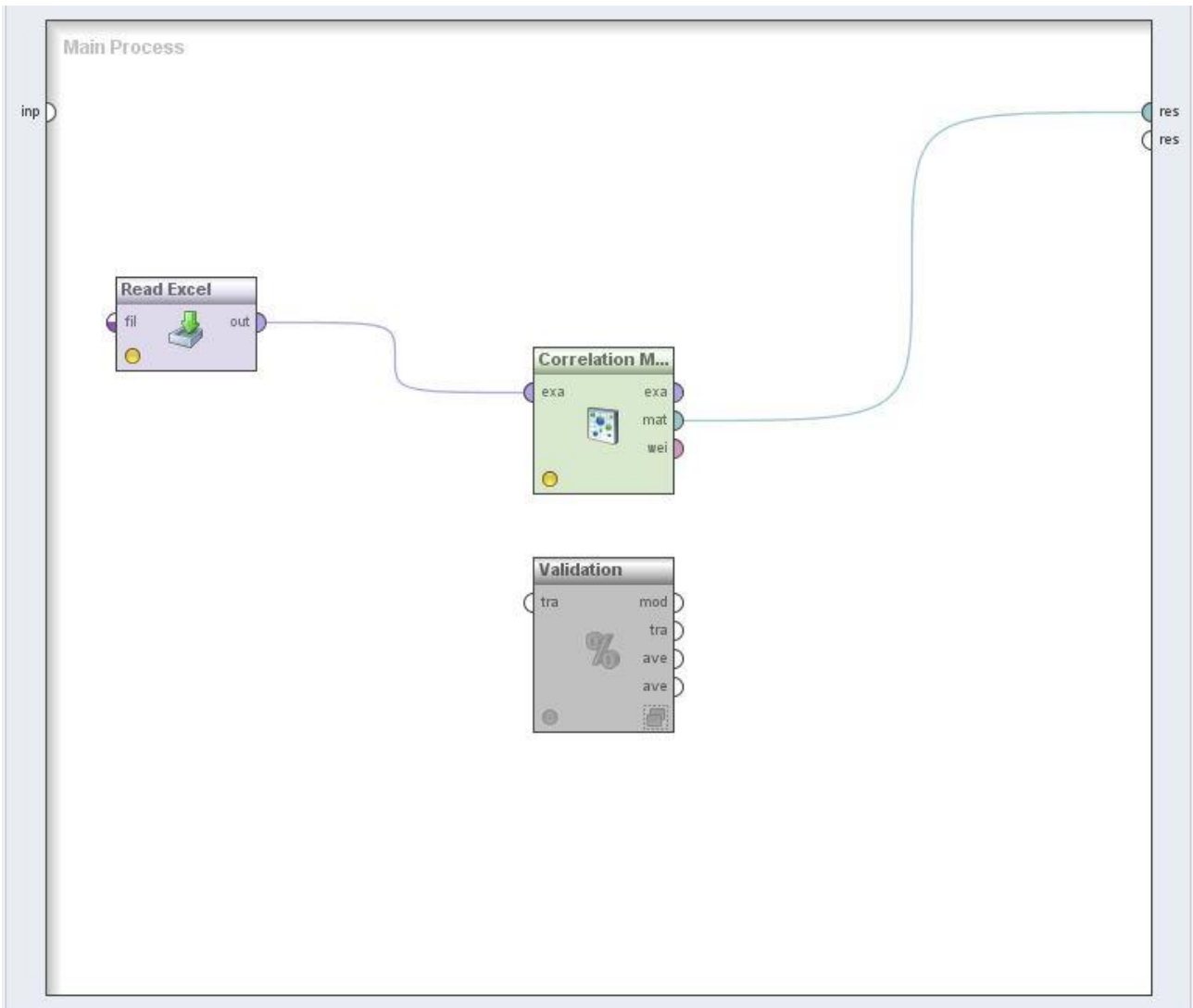
Figure 6. Correlation matrix
