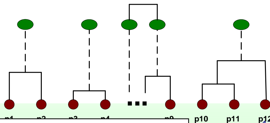
Proximity Matrix
