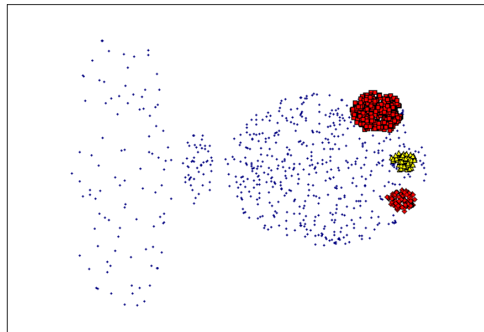
(MinPts=4, Eps=9.62)
