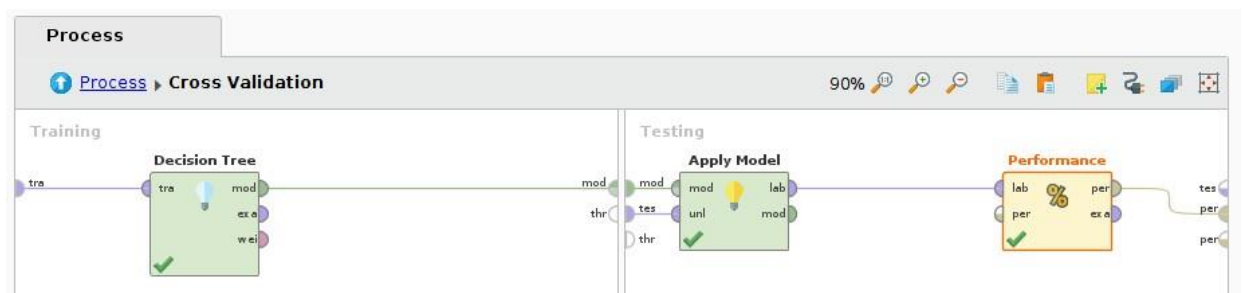
Figure 5. Validation subprocess. RapidMiner 9+
