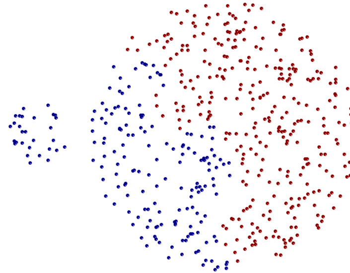
Two Clusters
