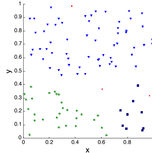
DBSCAN
