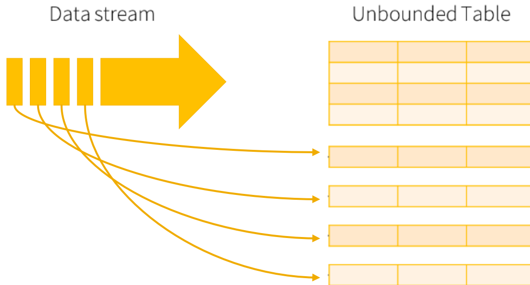
Data stream as an unbounded table
